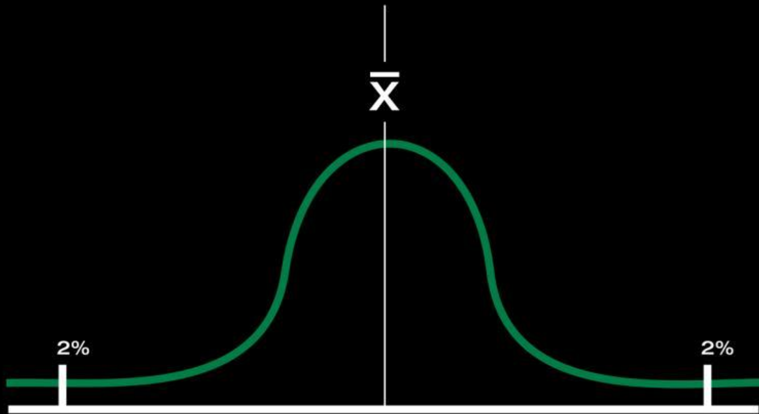
THE NORMAL DISTRIBUTION CURVE
